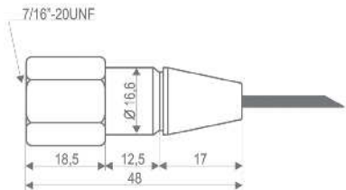
FEMALE FITTING
