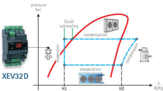
Pressure-enthalpy diagram shows the refrigeration cycle and the sub-cooling zone.
